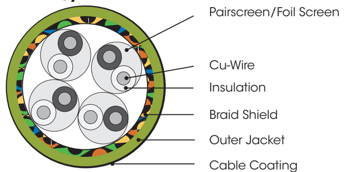
S/FTP
