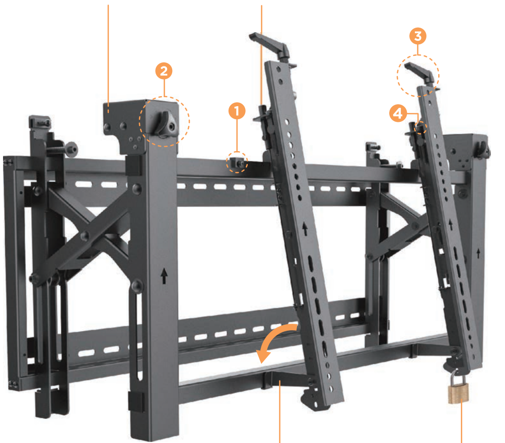
Kick-Stand Design provides 12° tilt for cable management and maintenance
